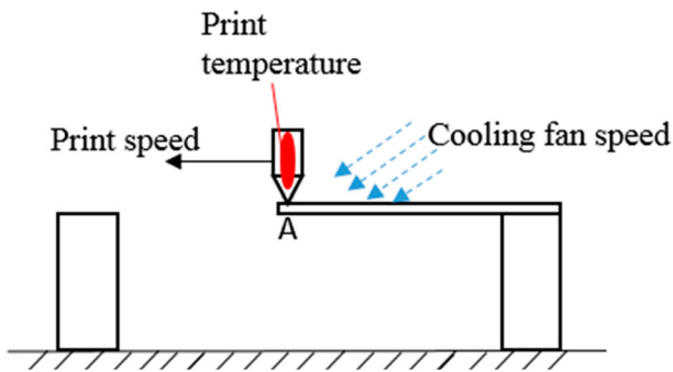
Figure 2. Illustration of effects of process parameters.
