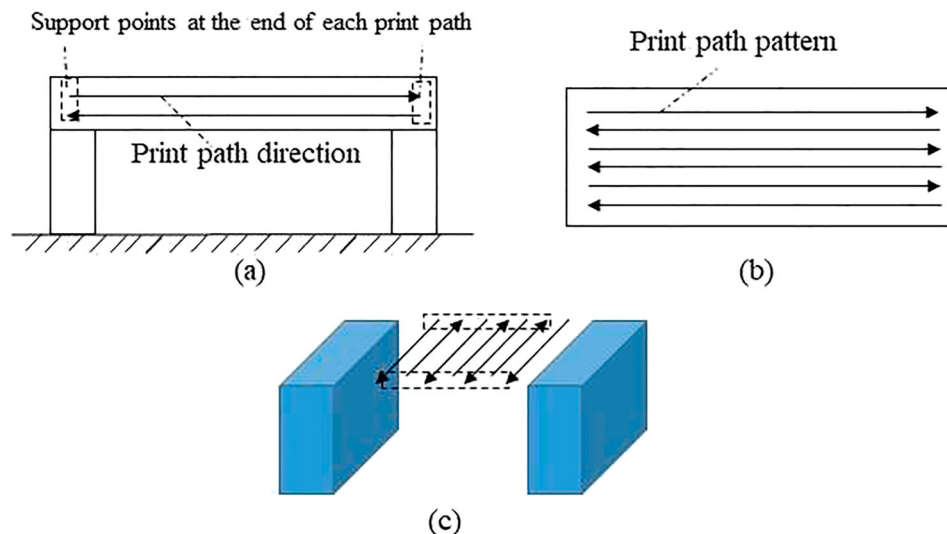
Figure 4. (a) Front view of print path; (b) top view of print path pattern; (c) no support points beneath the ends of each print path, this is unprintable.
