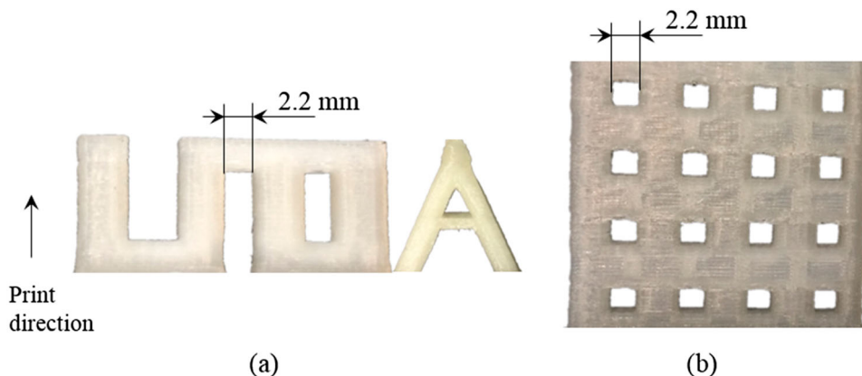
Figure 11. Printed ‘UOA’ and pane parts with satisfied bridge deformations (thickness of these parts is 2 mm).
