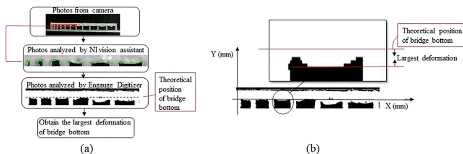
Figure 5. (a) Analysis programme of bridges; (b) definition of largest deformation in these bridges.
