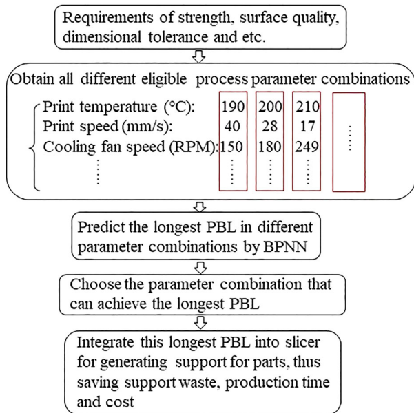
Figure 10. Framework of using BPNN for reducing support waste in additive manufacturing processes.
