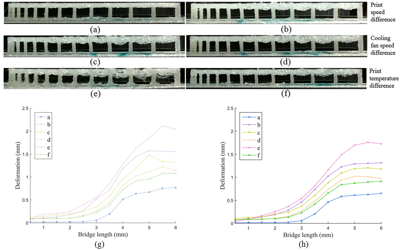
Figure 9. Samples printed in different conditions; (a) Part printed in print speed of 5 mm/s, cooling fan speed of 250 RPM, print temperature of 190°C; (b) Part printed in print speed of 95 mm/s, cooling fan speed of 250 RPM, print temperature of 190°C; (c) Part printed in cooling fan speed of 0 RPM, print speed of 35 mm/s, print temperature of 190°C; (d) Part printed in cooling fan speed of 250 RPM, print speed of 35 mm/s, print temperature of 190°C; (e) Part printed in print temperature of 220°C, cooling fan speed of 250 RPM, print speed of 35 mm/s; (f) Part printed in print temperature of 175°C, cooling fan speed of 250 RPM, print speed of 35 mm/s. (g) Largest deformations of the samples shown in (a)–(f). (h) Corresponding predictions from the developed ANN model for the samples shown in (a)–(f).
