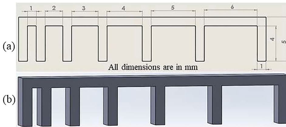
Figure 3. (a) 2D view of bridge (Unit: mm); (b) 3D view of bridge.
